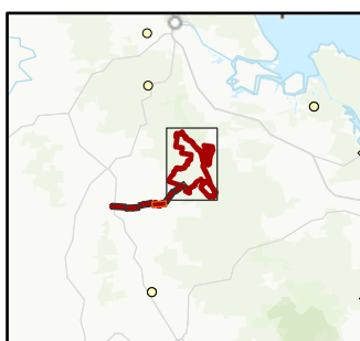
FIGURE 7.16D ORIENTAL CUCKOO POTENTIAL HABITAT
