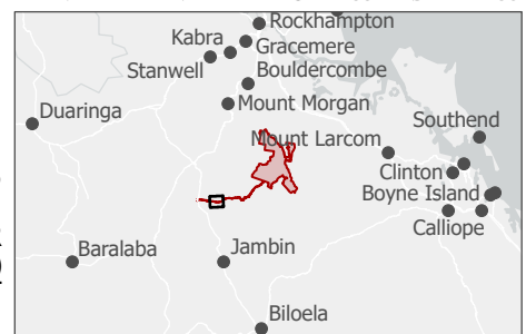
FIGURE 7.14B YELLOW-BELLIED GLIDER (SOUTH-EASTERN) HABITAT
