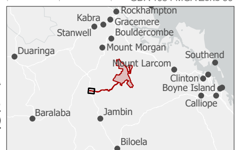
FIGURE 7.14A YELLOW-BELLIED GLIDER (SOUTH-EASTERN) HABITAT
