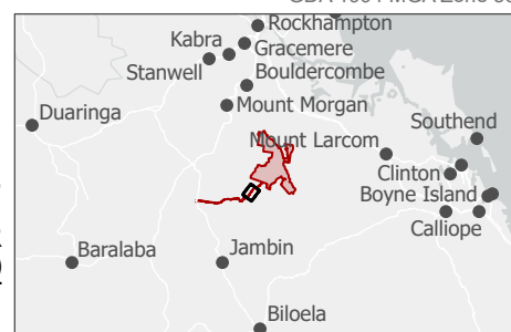
FIGURE 7.14E YELLOW-BELLIED GLIDER (SOUTH-EASTERN) HABITAT
