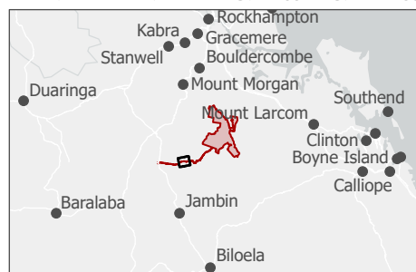
FIGURE 7.14C YELLOW-BELLIED GLIDER (SOUTH-EASTERN) HABITAT
