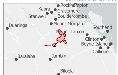
FIGURE 7.14D YELLOW-BELLIED GLIDER (SOUTH-EASTERN) HABITAT
