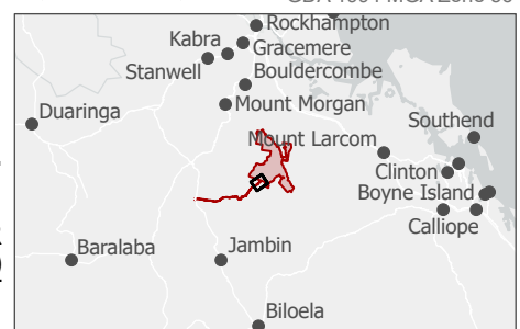
FIGURE 7.14F YELLOW-BELLIED GLIDER (SOUTH-EASTERN) HABITAT
