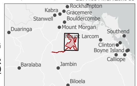
FIGURE 7.14G YELLOW-BELLIED GLIDER (SOUTH-EASTERN) HABITAT
